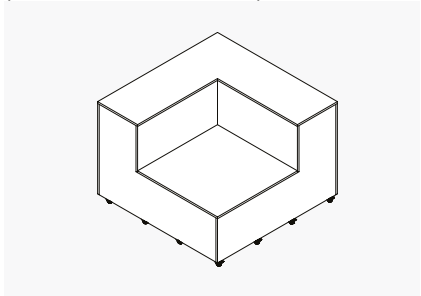
Module 12 with castors W: 1350 x D: 1350 x H: 940 mm (W: 53 x D: 53 x H: 37in)
