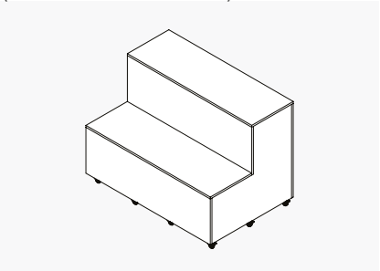
Module 9 Large with castors W: 1350 x D: 900 x H: 940 mm (W: 53 x D: 35 x H: 37in)
