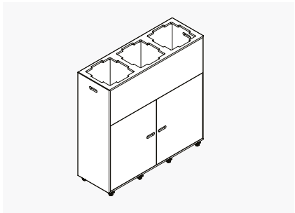
3 Box Planter 1350 storage and doors W: 1350 x D: 450 x H: 1350 mm (W: 53 x D: 18 x H: 53in)
