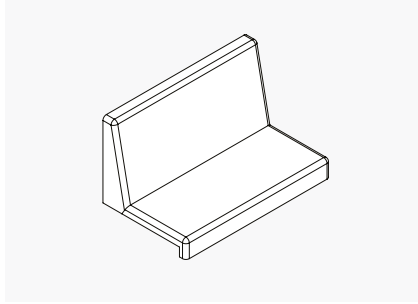
Double Full Seat square back W: 850 x D: 494 x H: 440 mm (W: 33 x D: 19 x H: 17in)
