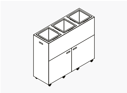
3 Box Planter 1125 storage and doors W: 1350 x D: 450 x H: 1125 mm (W: 53 x D: 18 x H: 44in)
