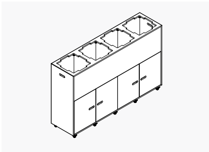
4 Box Planter 1125 storage and doors W: 1800 x D: 450 x H: 1125 mm (W: 71 x D: 18 x H: 44in)
