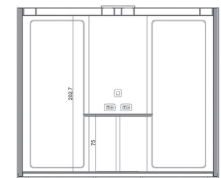
BUSYPOD XLarge plan section
