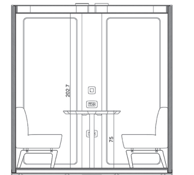
BUSYPOD Large section
