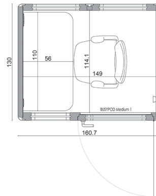
BUSYPOD Medium Work plan section
