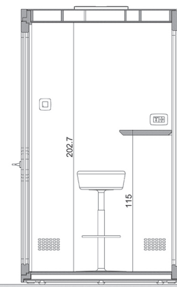
BUSYPOD Medium Meet section
