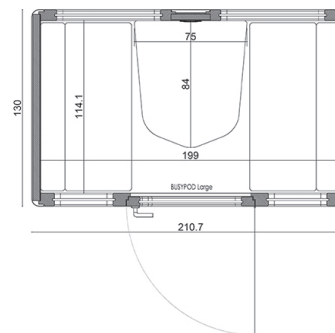
BUSYPOD Large plan section
