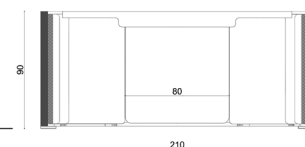
BUSYLOUNGE 2 person plan section
